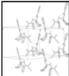
Fig. 2. The molecular packing diagram of the title compound showing intermolecular and intramolecular interactions by dashed lines.
