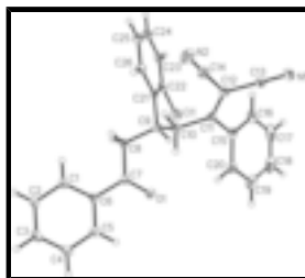
Fig. 1. The molecular structure drawing for the title compound; displacement ellipsoids are drawn at 20% probability level.
